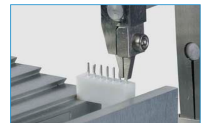
Torsion Testing
